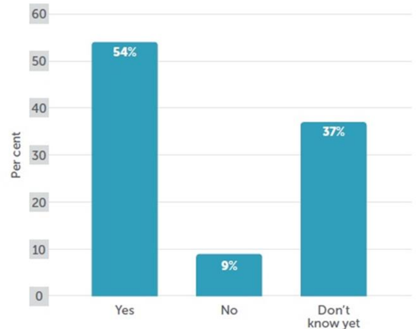
Graph 3 / Do you expect to deliver services with (or alongside) Community Rehabilitation Companies (CRCs)?
