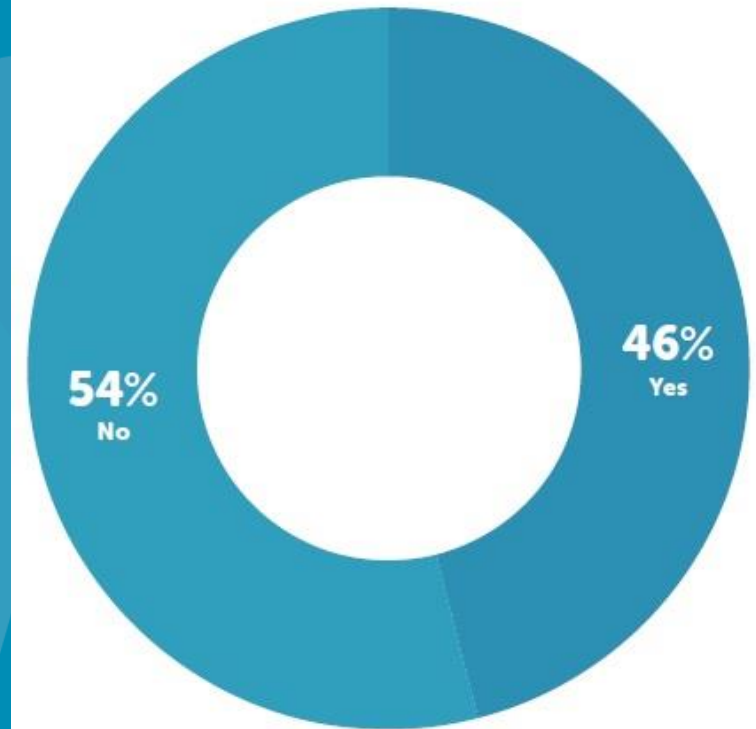
Graph 5 / Has your funding (contractual or grant funding) been affected by Transforming Rehabilitation?
